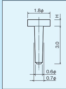
LYS-1-0.5~2
