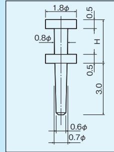
LYS-1-2.5~10
