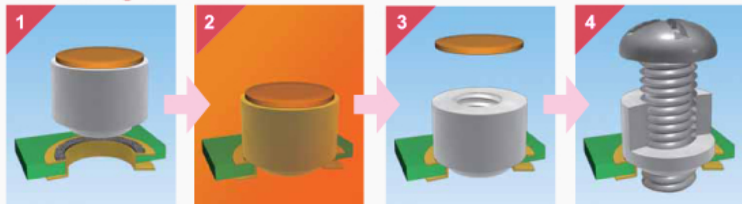
1 Pick and Place by Automatic Mounting Machine
